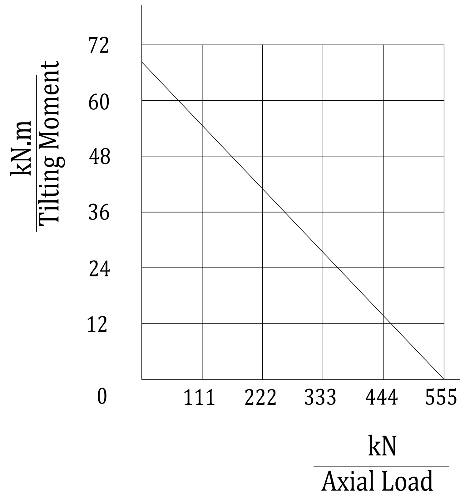
MOMENT LOAD CHART
